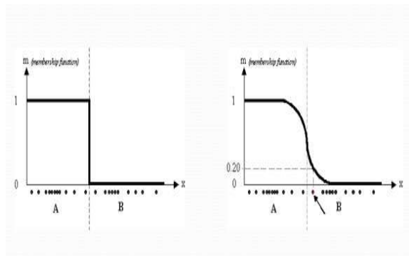
Fig. 4(a) – Hard Membership Function, Soft Membership Function.
