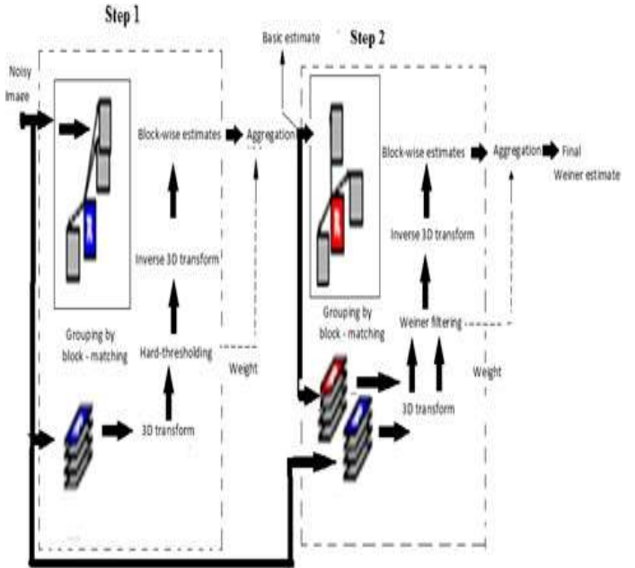
Fig. 3. Flowchart of the Proposed Image De-Noising Algorithm. the Operations Surrounded By Dashed Lines Are Repeated For Each Processed Block (Marked With R)
